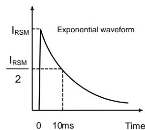
Figure 1. I_{RSM} waveform
