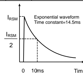
Figure 1. I_{RSM} waveform
