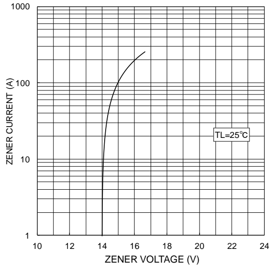
Typical zener characteristics
