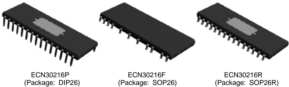
FIGURE 1.4.1 Packages of ECN30216
