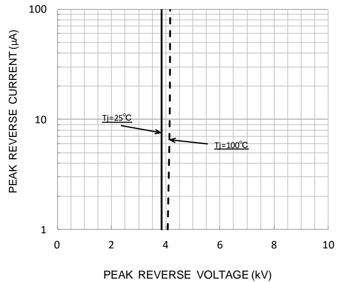
Typical Reverse Current characteristic ( I_r : 1 \mu A ~ 100 \mu A)
