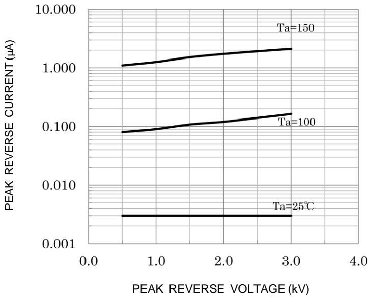
Typical Reverse Current characteristic ( I_r : 0.001 \mu A ~ 10 \mu A)
