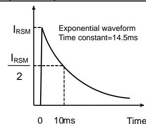
Figure 1. I_{RSM} waveform
