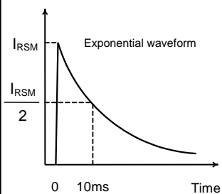
Figure 1. I_{RSM} waveform
