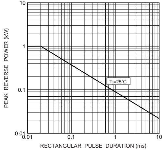
逆耐量特性 (非繰り返し) Typical reverse power characteristics (Non-repetitive)
