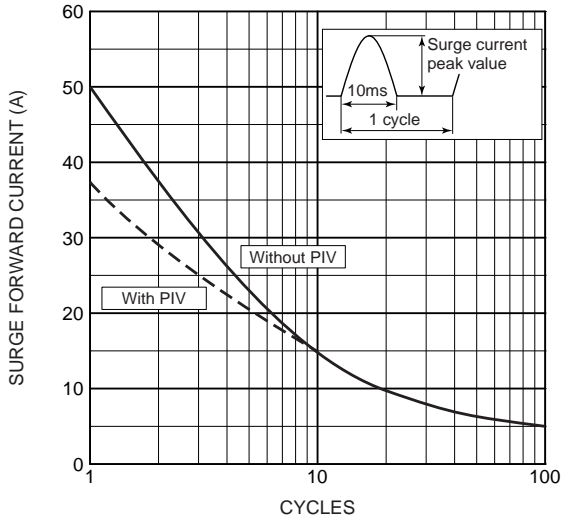
サージ順電流特性 (非繰り返し) Surge forward current characteristics (Non-repetitive)
