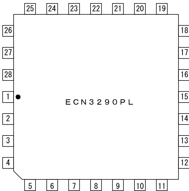
28pin J-Lead Package
