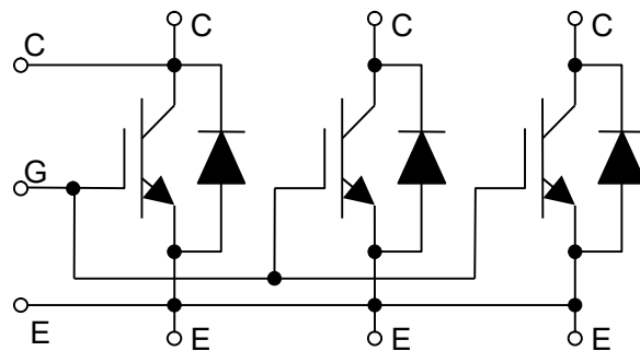
Fig.2 Circuit diagram
