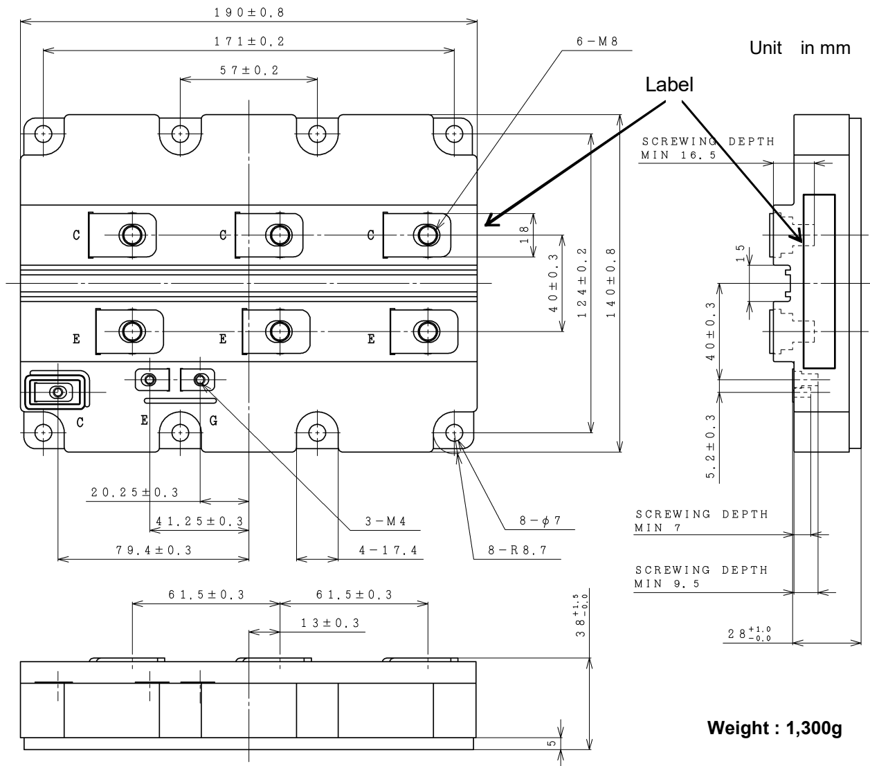
Fig.1 Outline Drawings
